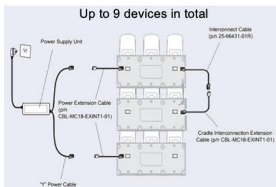
Figure 2: Fast charging with DC Y cable
